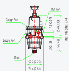
YT-200/205 manual drain
