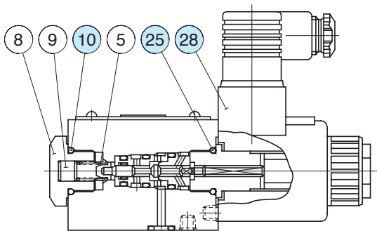
3 Port Valve
